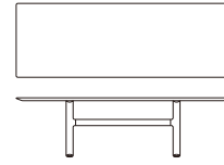
T-384 dining table W2600×D900×H720
